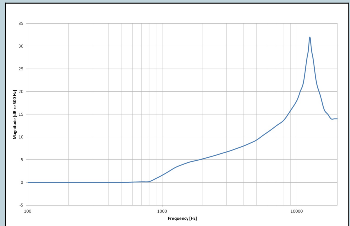
Typical frequency response GRAS Sound & Vibration reserves the right to change specifications and accessories without notice.
